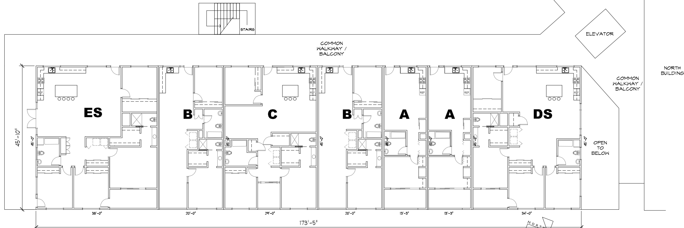
2 LEVELS 2 AND 3 SCALE: 1/8"=1'-0"
